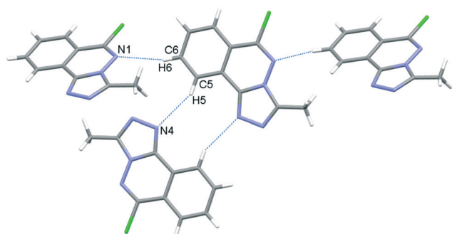
Fig. 3 C–H···N bonding motifs in 5 .
