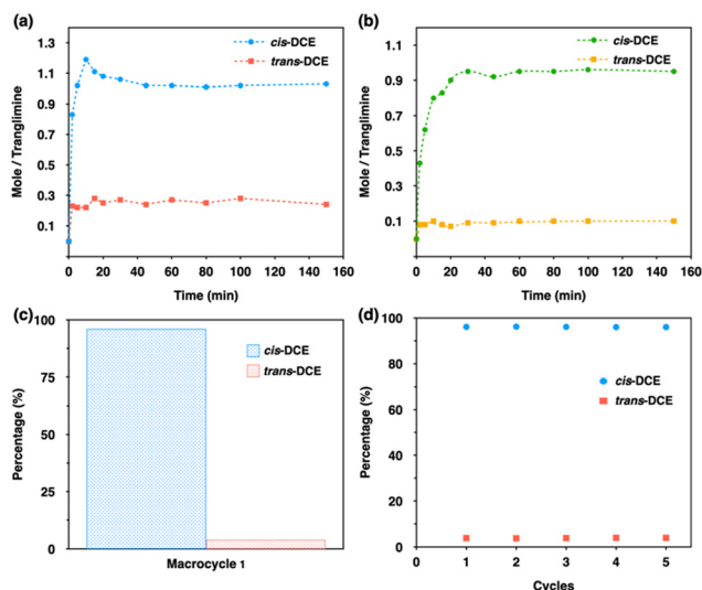
Fig. 4 (a) Time-dependent solid–vapor sorption plot of 1 \alpha for single-component cis - and trans -DCE. (b) Time-dependent solid–vapor sorption plot of 1 \alpha in cis/trans -DCE (1:1 v/v) mixture. (c) Relative uptake of cis - and trans -DCE over 1 h. (d) Relative uptake capacity of crystalline 1A towards cis/trans -DCE (1:1 v/v) mixture for 5 cycles.
