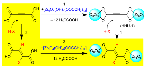
Scheme 7 Possible reaction mechanisms for the synthesis of Zr-HHU-2-X via the formation of hydrogen halide (HX, X = Cl, Br, I) and in situ hydrohalogenation of ADC after the formation of HHU-1 (route 1) or via a prior formation of a halofumarate linker and MOF formation with this linker in a second step (route 2). Adapted from ref. 134 with permission of the American Chemical Society, copyright 2019.
