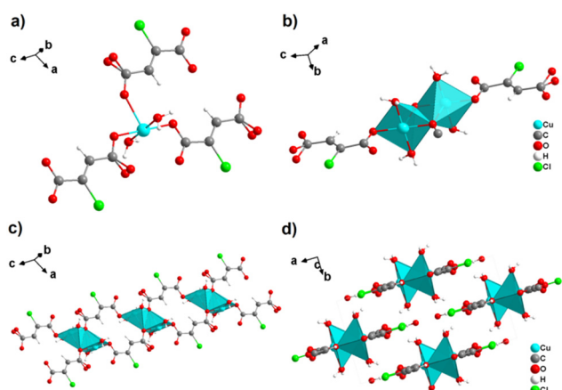
Fig. 43 Crystal structure of [\text{Cu}(\text{OOC}-\text{CH}=\text{Cl}-\text{COO})(\text{H}_2\text{O})_2]\cdot\text{H}_2\text{O} showing: (a) the coordination environment of \text{Cu}^{2+} , (b) the dinuclear building unit with connecting chlorofumarate linkers, (c) one-dimensional ribbon extending along [001] and (d) the packing of ribbons viewed along [001] . Note: one oxygen atom of the carboxylate group neighbouring the CH moiety is disordered over two (split) positions. Graphics redrawn from the cif file (CSD-Refcode LEHJIS). 133
