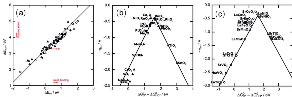
Fig. 3 (a) Adsorption energy of HOO* plotted against the adsorption energy of HO* on perovskite, rutile, anatase, \text{Mn}_x\text{O}_y , \text{Co}_3\text{O}_4 , and NiO oxides. (b) Trends for the OER activity on rutile, anatase, \text{Mn}_x\text{O}_y , \text{Co}_3\text{O}_4 , and NiO oxides. (c) Trends for the OER activity on perovskite. Reproduced with permission. 123 Copyright 2011, Wiley-VCH.
