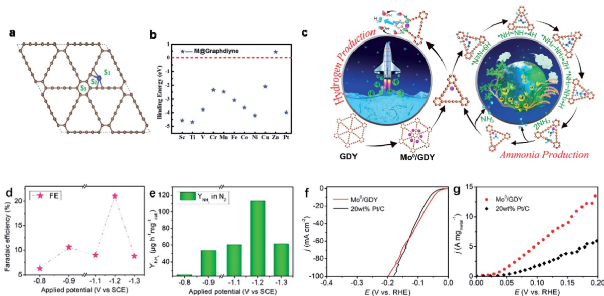
Fig. 11 (a) Different possible adsorption sites for the single TM atoms supported on GDY: (a) at the centre of the holes ( \text{S}_1 ), at the corner of the holes ( \text{S}_2 ) and at the centre of the hexatomic ring ( \text{S}_3 ). (b) The corresponding binding energies for adatoms absorbing on a single GDY layer. 136 Copyright 2019 Wiley-VCH. (c) Synthesis and structural configuration evolution of the catalysis process. ECNRR performance of \text{Mo}^0/\text{GDY} . (d) FEs and (e) \text{Y}_{\text{NH}_3} at different applied potentials in 0.1 \text{ M Na}_2\text{SO}_4 . HER performance characteristics. (f) Polarization curves and (g) mass activities of \text{Mo}^0/\text{GDY} and 20 wt% Pt/C. 137 Copyright 2019 American Chemical Society.
