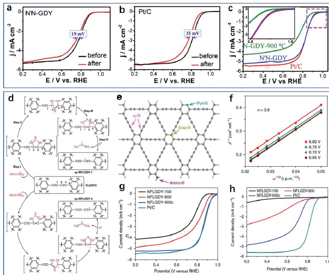
Fig. 4 Durability test of the (a) N'-N-GDY and (b) commercial Pt/C for 5000 CV cycles in \text{O}_2 -saturated 0.1 M KOH. (c) LSV curves of N-GDY-900 °C, N'-N-GDY, and commercial Pt/C at 1600 rpm in \text{O}_2 -saturated 0.1 M KOH. 104 Copyright 2017 American Chemical Society. (d) Synthesis of sp-N-doped few-layer GDY. (e) Geometries of N atoms in NFLGDY. (f) Corresponding Koutecky–Levich plots ( J^{-1} versus \omega^{-1/2} ). (g) Electro-catalytic ORR activity of NFLGDY and commercial Pt/C in \text{O}_2 -saturated 0.1 M KOH. (h) Electrochemical characterization of NFLGDY and commercial Pt/C for the ORR in \text{O}_2 -saturated 0.1 M \text{HClO}_4 . 105 Copyright 2018 Springer Nature Limited.
