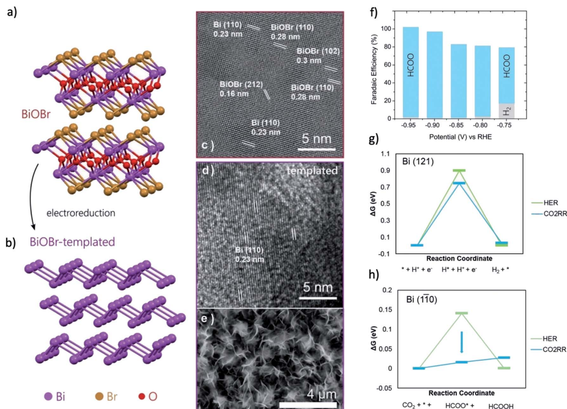
Fig. 11 Atomic structure of (a) BiOBr and (b) BiOBr-templated Bi catalyst after electroreduction. HRTEM of BiOBr (c) before and (d) after electroreduction reveal the selective reconstruction into Bi. (e) SEMs of samples after reaction reveal a 2D petal-like layered arrangement. (f) CO 2 RR product distribution of BiOBr-templated catalyst for different operating potentials. Formate is the only product at <−0.75 V. (g and h) The reaction energy diagram for HER and CO 2 RR on Bi (121) and Bi (110) facets. Adapted with permission from ref. 152 Copyright © 2018, Wiley-VCH.
