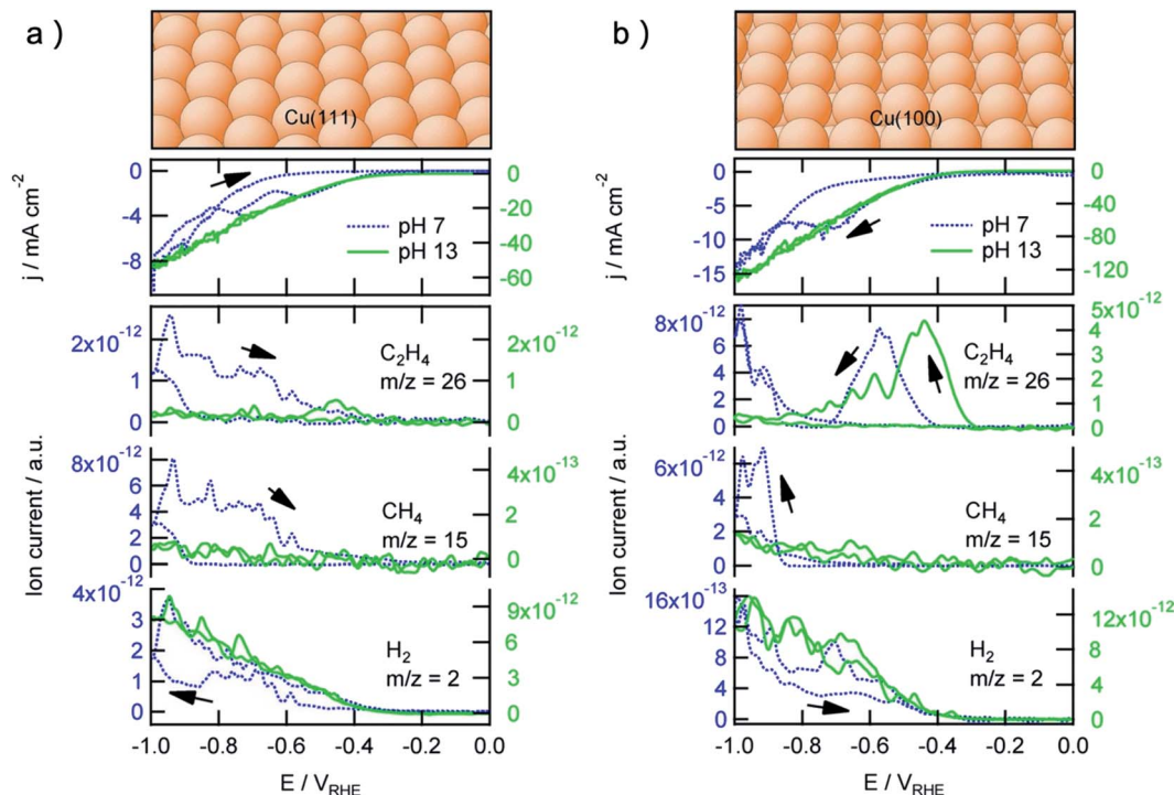
Fig. 10 (a) Top: (111) facet of the copper fcc crystal. Middle: The catalytic current measured by cyclic voltammograms for the reduction of a saturated solution of CO ( \sim 1 mM) on Cu(111) in phosphate buffer (pH 7) and NaOH solution (pH 13). Bottom: Products of CO reduction at different potential measured by online electrochemical mass spectrometry. (b) Top: (100) facet of the copper fcc crystal. Middle: The catalytic current measured by cyclic voltammograms for the reduction of a saturated solution of CO ( \sim 1 mM) on Cu(100) in phosphate buffer (pH 7) and NaOH solution (pH 13). Bottom: Products of CO reduction at different potential measured by online electrochemical mass spectrometry. Adapted with permission from ref. 15 Copyright © 2012, American Chemical Society.
