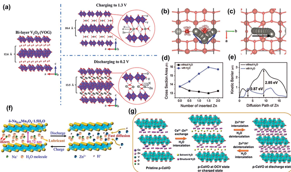
Fig. 3 (a) The proposed crystal structures of pristine \text{V}_2\text{O}_5 \cdot n\text{H}_2\text{O} , and \text{V}_2\text{O}_5 \cdot n\text{H}_2\text{O} after charging to 1.3 V, and discharging to 0.2 V. Reproduced with permission. 47 Copyright 2017, Wiley-VCH. Diffusion paths of Zn ions (b) with and (c) without water (projected down [001]). (d) Change in the cross-sectional area of the diffusion path during Zn intercalation with and without water. (e) Calculated diffusion barriers for paths in (b) and (c). (b–e) Reproduced with permission. 72 Copyright 2019, Wiley-VCH. (f) Schematic of Na ion and water molecule pre-intercalated \delta\text{-MnO}_2 for Zn ion storage. Reproduced with permission. 76 Copyright 2019, American Chemical Society. (g) Schematic illustration of the reaction mechanism of p-CaVO. Reproduced with permission. 78 Copyright 2019, American Chemical Society.
