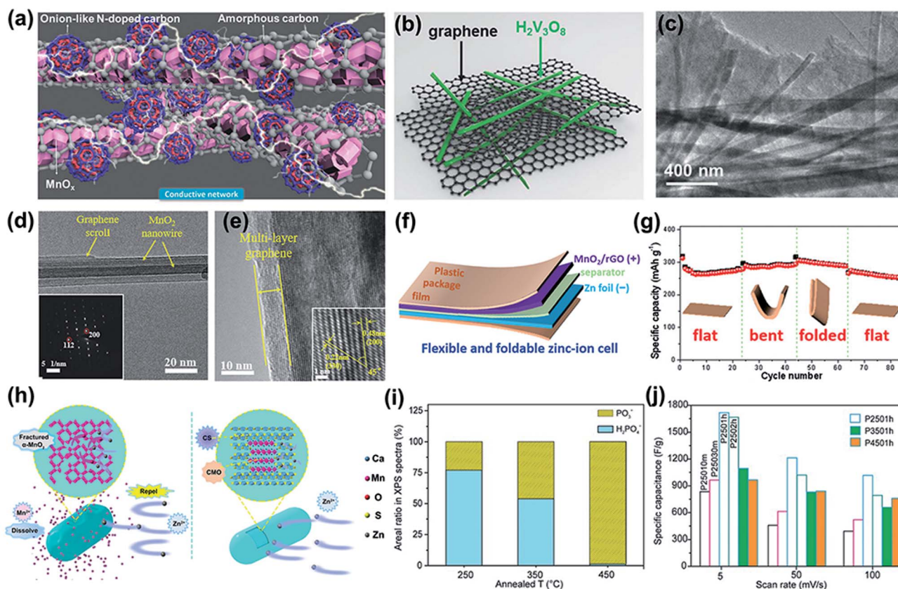
Fig. 8 (a) Schematic of the structure of MnO x @N-C nanorods. Reproduced with permission. 117 Copyright 2018, Wiley. (b) Schematic illustration of the structure of H 2 V 3 O 8 NW/graphene. (c) TEM image of H 2 V 3 O 8 NWs on graphene films. (b and c) Reproduced with permission. 51 Copyright 2018, Wiley. (d) TEM images and SAED (inset) of α-MnO 2 /graphene scrolls. (e) The HRTEM of α-MnO 2 /graphene scrolls. (d and e) Reproduced with permission. 126 Copyright 2018, Wiley. (f) Schematic illustration of a flexible and foldable ZIB cell. (g) Cycling stability of the ZIB cell under different mechanical deformations. (f and g) Reproduced with permission. 129 Copyright 2020, Wiley. (h) The battery reaction mechanism schematic diagram of α-MnO 2 and Ca 2 MnO 4 . Reproduced with permission. 131 Copyright 2019, American Chemical Society. (i) Area% change of H 2 PO 4 - and PO 3 - at the surface of PCO as a function of annealed temperature. (j) Specific capacitances of different PCO samples prepared under various conditions as a function of scan rate. (i and j) Reproduced with permission. 132 Copyright 2016, Wiley.
