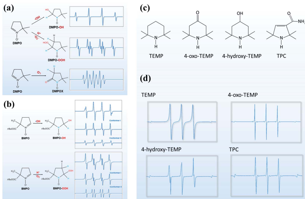
Fig. 12 (a) Structures and simulated EPR signals of DMPO-HO• and DMPO-HOO• adducts formed by trapping HO• and \text{O}_2^{\bullet-} with DMPO and DMPOX formed by oxidation of DMPO with \text{O}_3 . (b) Structures and EPR signals of BMPO-HO• and BMPO-HOO• adducts formed by trapping HO• and \text{O}_2^{\bullet-} with BMPO. Adapted with permission from ref. 16. Copyright 2020, American Chemical Society. (c) Chemical structures of four sterically hindered amines. (d) EPR signals of nitroxide radicals formed by trapping ^1\text{O}_2 with four sterically hindered amines. Reproduced with permission from ref. 230. Copyright 2017, Royal Society of Chemistry. Reproduced with permission from ref. 231. Copyright 2011, Royal Society of Chemistry.
