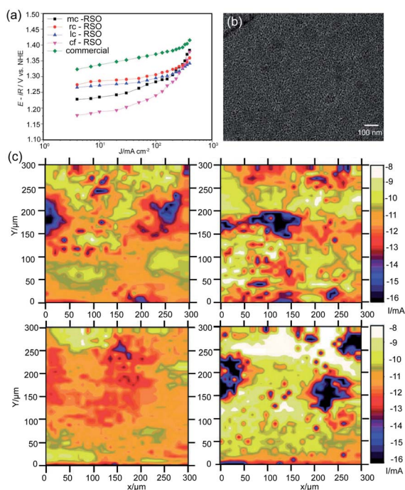
Fig. 8 (a) Galvanostatic polarization curves in 3.5 \text{ M} , \text{pH} = 3 \text{NaCl} solution and 80^\circ \text{C} for different \text{Ru}_{0.3}\text{Sn}_{0.7}\text{O}_2 coating morphologies ( 5.78 \text{ g}_{\text{Ru}} \text{ m}^{-2} ) and the commercial \text{Ru}_{0.3}\text{Ti}_{0.7}\text{O}_2 coating ( 12.1 \text{ g}_{\text{Ru}} \text{ m}^{-2} ). (b) SEM image of the \text{Ru}_{0.3}\text{Sn}_{0.7}\text{O}_2 coating with crack-free surface microstructure. (c) SECM activity images of different \text{Ru}_{0.3}\text{Sn}_{0.7}\text{O}_2 coatings in 5 \text{ M} , \text{pH} = 2 \text{NaCl} solution at room temperature. The applied potentials are 1.6 \text{ V} for the sample and 1.15 \text{ V vs. SHE} for the Pt tip. (Left top) mud-crack, (right top) reduced-crack, (left bottom) less-crack, and (right bottom) crack-free. Reproduced with permission. 45 Copyright 2012, Royal Society of Chemistry.
