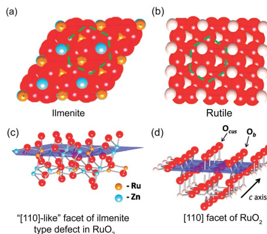
Fig. 6 (a) Atomic close packing model of the ilmenite structure and (b) rutile structure. (c) Spatial ilmenite structure of the active \text{RuO}_2 (110) surface. (d) Spatial rutile structure of the active \text{RuO}_2 (110) surface. Reproduced with permission. 44 Copyright 2011, American Chemical Society.
