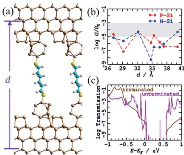
Fig. 4 Modelling the STMBJ experiment, using regular unterminated silicon tips on each unterminated electrode. (a) 2D ( 3 \times 3 ) model for tips spanned by \text{Si}(\text{CH}_2)_6\text{S} at d = 37.37 \text{ \AA} ; Si-brown, S-yellow, C-cyan, H-white. (b) Conductivity at zero voltage for P-type and N-type silicon at 0 K; the shaded region shows the observed conductance found throughout extensions of 3–10 Å for P-type Si. See ESI† Fig. S4 for more information. (c) Comparison of the transmission for P-type Si, as a function of electron energy from the Fermi energy, at d = 32.17 \text{ \AA} , from this unterminated series to that for the analogous terminated structure (Fig. 3, ESI† Fig. S3).
