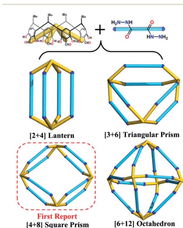
Scheme 1 Self-assembly of organic cages constructed from the tetraformyl C4RACHO cavitand and dihydrazide linkers.
