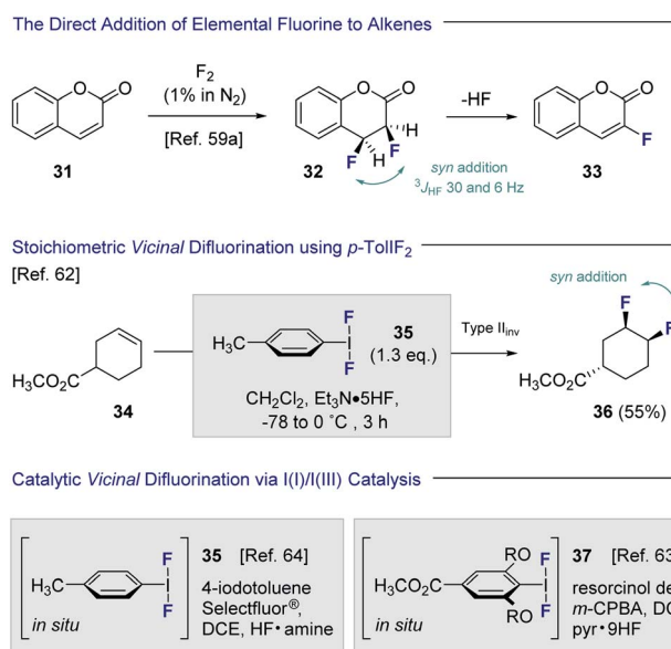
Fig. 8 The direct vicinal difluorination of alkenes via I(I)/I(III) catalysis.
