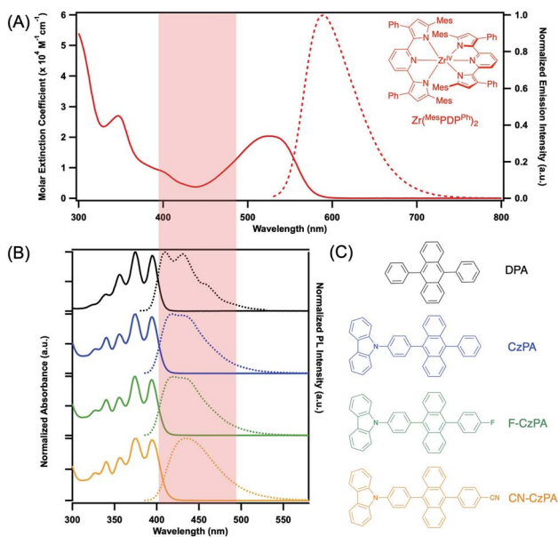
Fig. 2 (A) Electronic absorption (solid line) and photoluminescence (dashed line) spectra of Zr^{(Mes)PDP^{Ph}}_2 in THF. (B) Normalized absorption (solid lines) and photoluminescence (dashed lines) spectra of DPA (black), CzPA (blue), F-CzPA (green) and CN-CzPA (orange). The red shaded area shows a small spectral overlap between photoluminescence of acceptors and absorbance of Zr^{(Mes)PDP^{Ph}}_2 , indicating minimal reabsorption of upconverted fluorescence by the sensitizer. (C) Chemical structures of DPA (black), CzPA (blue), F-CzPA (green) and CN-CzPA (orange).
