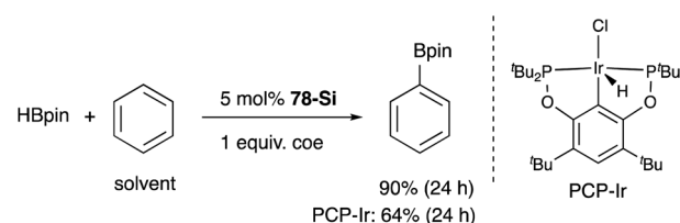
Scheme 36 \text{sp}^2\text{C} –H borylation catalyzed by the bis(silylene)–Ir complex 78–Si.
