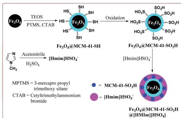
Scheme 48 Preparation of Fe 3 O 4 @MCM-41-SO 3 H@[HmIm][HSO 4 ] nanocatalyst.
