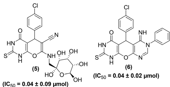
Fig. 5 Chemical structures of selected pyrano[2,3-d]pyrimidines (5 and 6).
