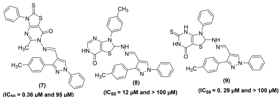
Fig. 6 Chemical structures of substituted 1H-pyrazolyl-thiazolo[4,5-d]pyrimidines (7–9).
