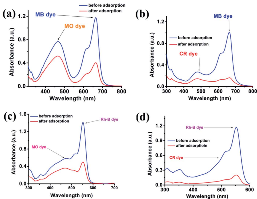
Fig. 8 Adsorption plots of MB (a and b) and Rh-B (c and d) in the presence of MO and CR using the \{\text{Fe}_3\} cluster as the adsorbent.
