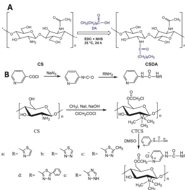
Fig. 25 Functionalization of chitosan scaffolds. A. Introduction of decanoic acid (DA) via NHS activation of the carboxylic acid of DA followed by reaction with the amine groups of chitosan. Reprinted from ref. 138 with permission from Elsevier, copyright (2019). B. Conjugation of urea compounds to the chitosan scaffold via chloroacetylation of the primary hydroxyls on the chitosan chain with 2-chloroacetyl chloride followed by conjugation of the urea compounds through reaction with the nitrogen of the heterocyclic urea compounds. Reprinted from ref. 120 with permission from Elsevier, copyright (2019).
