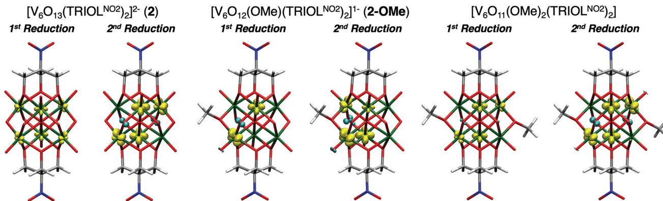
Fig. 7 Spin density of reduced 2 , 2-OMe , and para -[V 6 O 11 (OMe) 2 (TRIOLNO 2 ) 2 ] at M06/def2-TZVP//M06-L/def2-TZVP,def2-SVP level of theory. Vanadium in dark green, oxygen in red, nitrogen in blue, carbon in grey, and hydrogen in white. Alpha spin density in yellow and beta spin density in cyan. Isosurface = 0.4. Additional spin density plots for reduced variants of 1-OMe and meta - 1-(OMe) 2 can be found in Fig. S17.†
