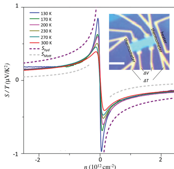
Fig. 15 Measured S/T_e as a function of charge carrier density n at different temperatures. The grey and purple curves represent S_{\text{Mott}}/T_e and S_{\text{hyd}}/T_e , respectively. The inset shows a typical device used to measure S , where the scale bar corresponds to 2\text{ }\mu\text{m} . The figure is adapted with permission from ref. 190 (Copyright 2016 American Physical Society).
