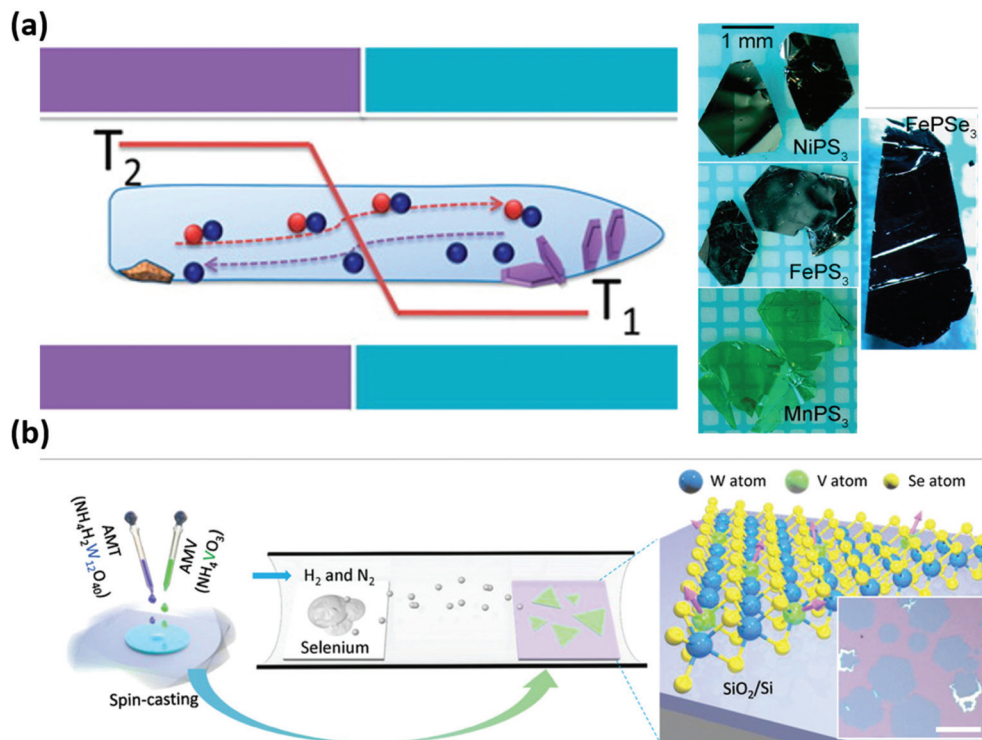
Fig. 4 Reported growth methods for 2D magnets: CVD and CVT. (a) CVT growth of metal phosphochalcogenides. The sketch depicts the reaction, where the halogen gas transports the elements from the hot to the cold side via convection. 146 Reproduced with permission from ref. 146. Copyright 2016 American Chemical Society. (b) CVD of V-doped \text{WSe}_2 . The mixed precursors react with Se on the \text{SiO}_2 surface into ferromagnetic V- \text{WSe}_2 . 147 Scale bar is 50 \mu\text{m} . Reproduced with permission from ref. 147. Copyright 2020 John Wiley and Sons.
