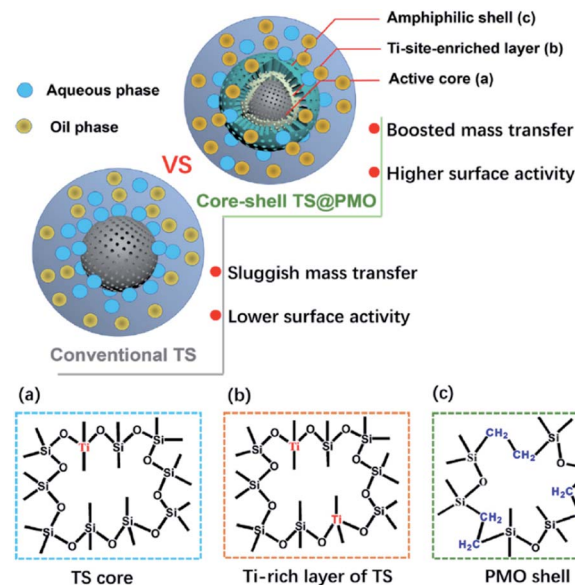
Fig. 4 Illustration of TS and TS@PMO showing the merits of material design with an amphiphilic shell and surface-Ti-enriched core (a), (b), and (c) indicate the skeleton structure of the TS core and PMO shell; note: (b) is the outer layer of (a). 68 Reproduced with permission. 68 Copyright 2021, Elsevier.
