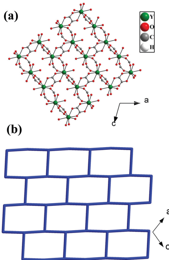
Fig. 1 (a) The 2D structure of [\text{Y}(\text{tp})(\text{ox})_{0.5}(\text{H}_2\text{O})_2]\cdot\text{H}_2\text{O}\cdot\mathbf{1} , formed by the connectivity of \text{Y}^{3+} ions and carboxylates of terephthalates and oxalates, (b) the 2D brick-wall topology based on three-connected \text{Y}^{3+} nodes.
