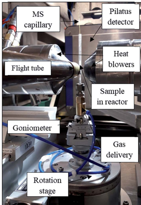
Fig. 1 Photograph of the setup used for the experiment at ID31 at the ESRF.
