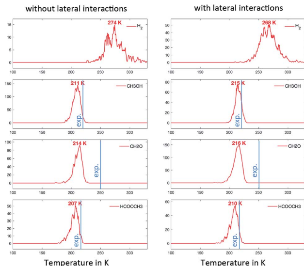
Fig. 4 TPO spectra of methanol on Au(111) for scenario #1. The temperature ramp is 10\text{ K s}^{-1} . The initial coverage in \text{CH}_3\text{O} is 0.1\text{ ML} . The blue line corresponds to the approximate position of the experimental peak.
