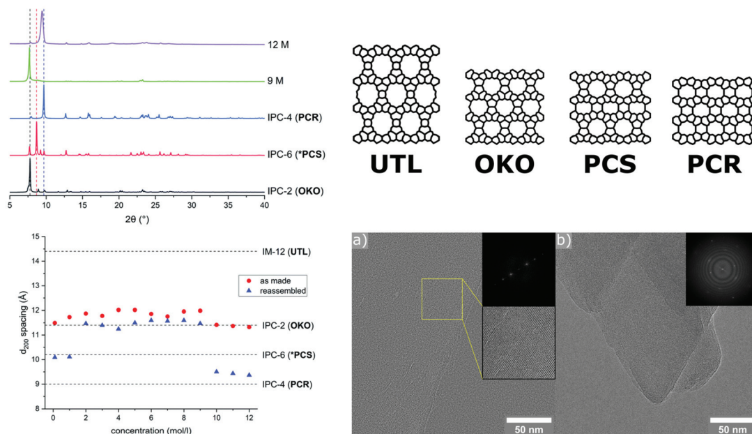
Fig. 8 Hydrolysis of zeolite UTL using a ball milling assisted method using comparatively low amounts of hydrochloric acid. PXRD patterns and d_{200} -spacing vs. acid concentration are shown on the left-hand side. The right panel shows the known structures of the parent zeolite UTL and relevant daughter phases, as well as TEM images of materials obtained with 25 mL 12 M HCl, showing lattice fringes indicative of the PCR framework. Adapted and reproduced from ref. 126 with permission from the Royal Society of Chemistry.
