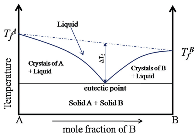
Fig. 1 Schematic phase diagram of a two component eutectic mixture (adapted from ref. 20).
