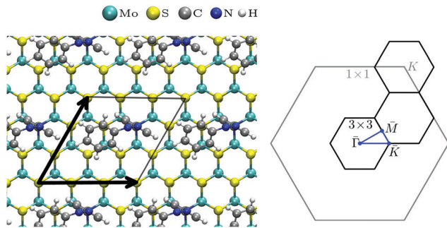
(a) Geometry and Brillouin zone of 3 \times 3 supercell (with cis -AAB).
