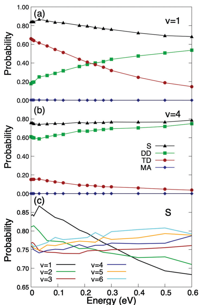
Fig. 3 Quasi-classical O 2 ( v , J = 1) reaction probabilities on Cu/Ru(0001) as a function of the incidence energy, for a surface temperature T_s = 350 K. (a) Vibrational state v = 1; (b) v = 4; (c) total sticking probabilities for vibrational states v = 1 to v = 6. S stands for total sticking probability, DD for direct dissociation, TD for trapping dissociation, and MA for molecular adsorption.
