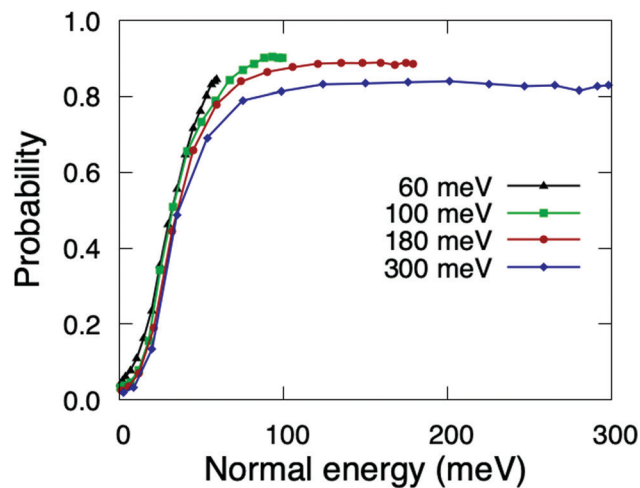
Fig. 5 Quasi-classical total sticking probabilities for O_2(v = 0, J = 0) on Cu_{1ML}/Ru(0001) as a function of the normal energy.
