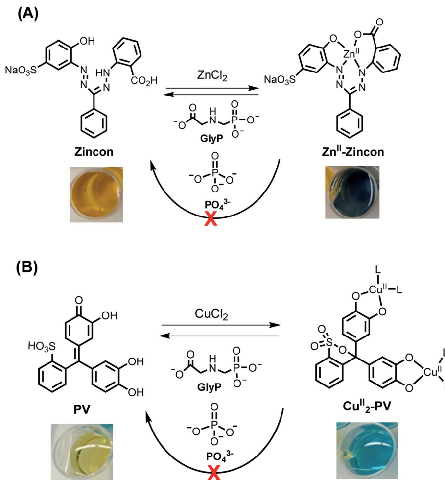
Fig. 4 Schematic representation and changes of the color of reactions between Zn II -zincon (30 \mu M; (A)) or Cu II -PV (30 \mu M; (B)) and GlyP (10 equiv.) or PO 4 3- (10 equiv.).
