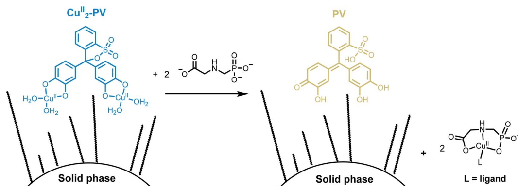
Fig. 2 Schematic representation of detection of GlyP with an immobilized \text{Cu}^{\text{II}}\text{-PV} complex by an indicator displacement assay using solid phase extraction.
