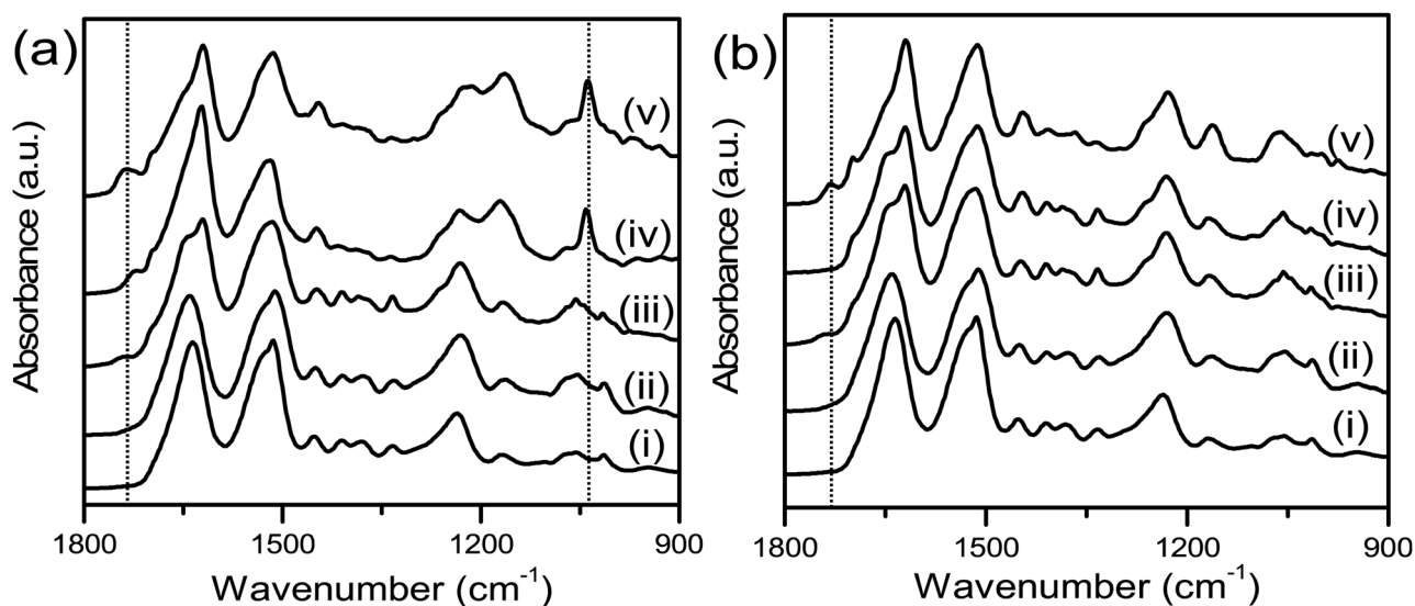
Fig. 1 (a) ATR-FTIR spectra of (i) unmodified SF ( SF_{As\text{ Cast}} ), (ii) SF_{EO} , (iii) SF_{OX} , (iv) SF_{EO\text{-zwitter}} , (v) SF_{OX\text{-zwitter}} , and (b) ATR-FTIR spectra of (i) unmodified SF ( SF_{As\text{ Cast}} ), (ii) SF_{EO} , (iii) SF_{OX} , (iv) SF_{EO\text{-PEG}} , (v) SF_{OX\text{-PEG}} . Vertical dashed reference lines in (a) correspond to S=O stretching at 1040\text{ cm}^{-1} and ester C=O stretching at 1735\text{ cm}^{-1} , and the dashed reference line in (b) corresponds to ester C=O stretching at 1735\text{ cm}^{-1} .
