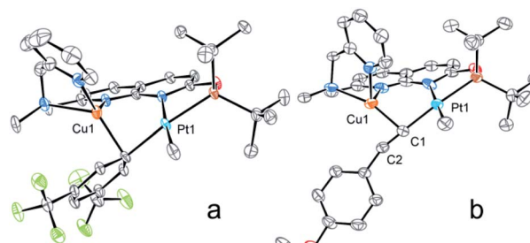
Fig. 4 ORTEP of 6[\text{B}(\text{Ar}^{\text{F}})_4] (a) and 7[\text{BF}_4] (b) at the 50% probability level. Hydrogen atoms, counterions, and solvent molecules together with the minor disorder component for 7[\text{BF}_4] are omitted for clarity.
