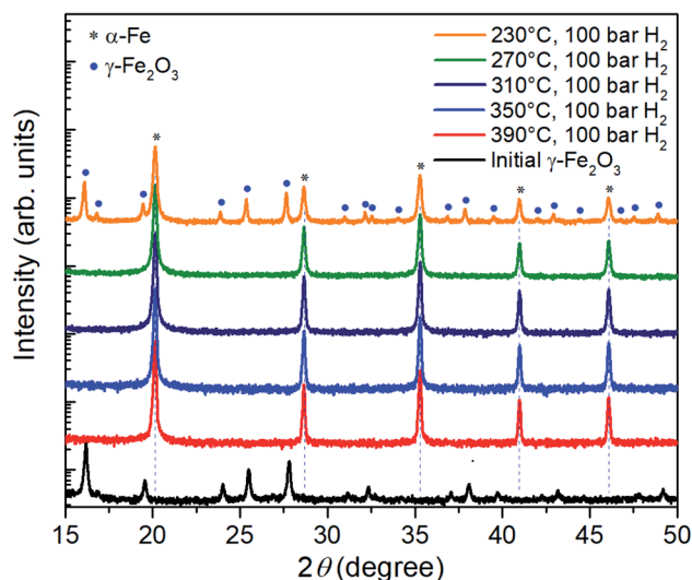
Fig. 2 XRD patterns of the \gamma\text{-Fe}_2\text{O}_3 nanoparticle powder before and after three-hour reduction in hydrogen at a pressure of 100 bar and temperatures between 230 °C and 390 °C.
