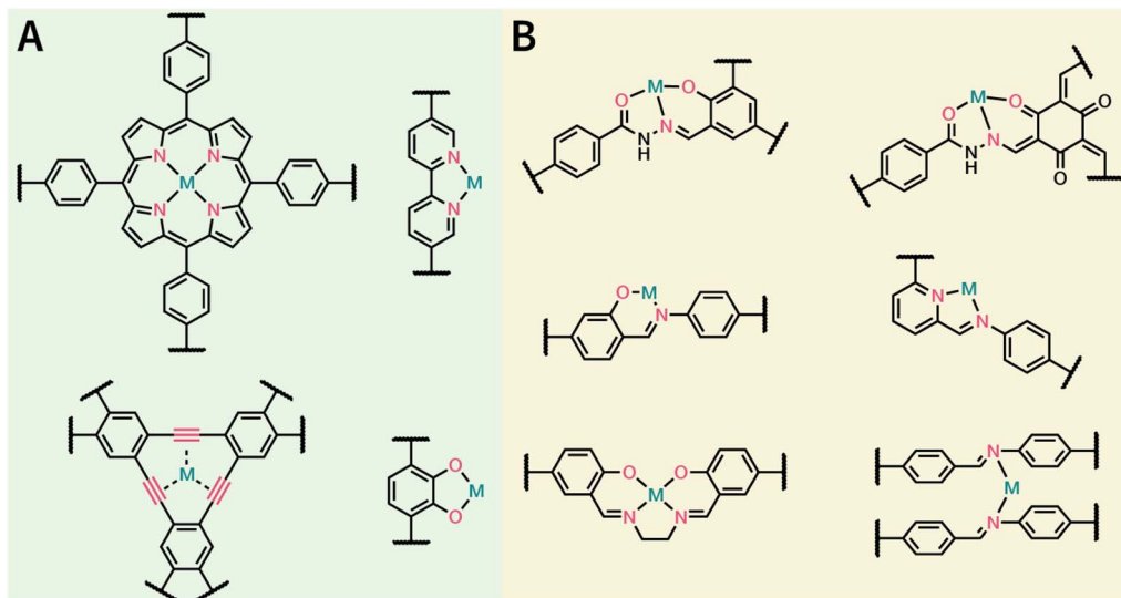
Fig. 63 Representative examples of the post-synthesis coordination modification of COFs. (A) Metal coordination sites on the monomer. (B) Metal coordination sites on linkages.
