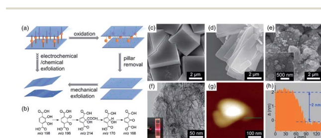
Fig. 4 (a) Illustration of the synthetic process of 2D MOFs by using the electrochemical/chemical exfoliation method and (b) a possible oxidative transformation route from \text{H}_4\text{dhbdc} to a species with m/z 168. SEM images of (c) 3D-Co, (d) 2D-Co, and (e) 2D-Co-NS. (f) TEM image of 2D-Co-NS (inset: Tyndall effect of a colloidal solution). (g) AFM image and (h) the corresponding height profile of 2D-Co-NS. Reproduced with permission. 77 Copyright©2018 WILEY-VCH Verlag GmbH & Co. KGaA.
