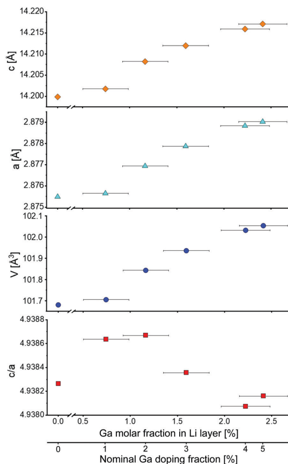
Fig. 3 Lattice parameters a and c , unit cell volume V and c/a ratio as a function of Ga content in the Li layer (as determined by Rietveld refinement). The bottom x -axis indicates the nominal Ga doping. All y -error bars are smaller than the data points.
