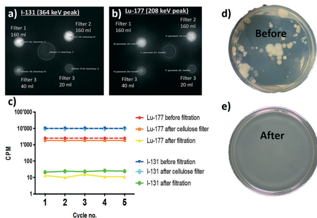
Fig. 4 (a) Planar scintigraphy of I-131 and (b) Lu-177 filters after filtration of increasing volumes. (c) Five gamma counter measurements for each filtrate. Biological contamination in the wastewater: wastewater plated on LB-agarose gel (d) before and (e) after filtration, respectively.
