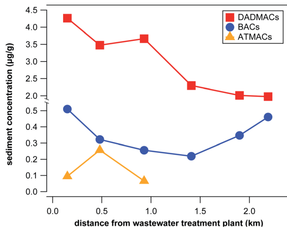
Fig. 3 Approximate total concentrations (all targets and suspects combined) of DADMACs (red squares), BACs (blue circles), and ATMACs (yellow triangles) in µg per g dry surface sediment with increasing distance from the only WWTP outlet in Lake Winona.
