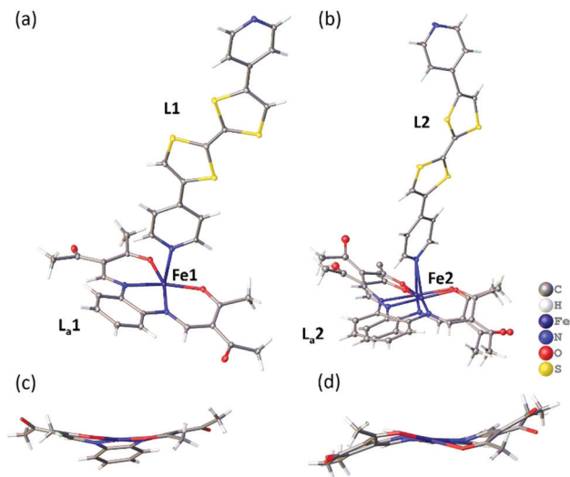
Fig. 1 Structural image of the asymmetric unit (100 K) of [\text{FeL}_a(\text{py}_2\text{TTF})]_n showing the distinct fragments composed of (a) Fe1-L1-L a 1 and (b) Fe2-L2-L a 2 . (c & d) show the umbrella and meso conformations of the L a 1 and L a 2 equatorial ligands. Thermal ellipsoid plot (50% probability); solvent molecules omitted for clarity.
