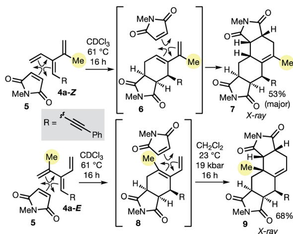
Scheme 2 DTDA sequences on each of the two diastereomers of [3] dendralene 4a grants access to constitutional isomers of a \Delta^{1(9)} -octalin 7 and 9 . All four cycloadditions are endo -selective and the second of each sequence exhibits \pi -diastereofacial selectivity.
