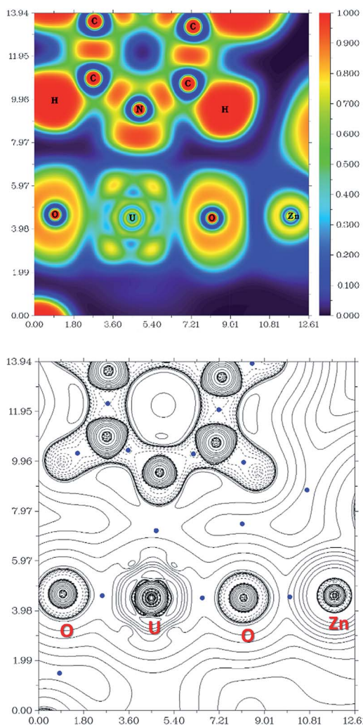
Fig. 9 Electron Localisation Function (ELF) diagram (top) and \nabla^2\rho contour line diagram (bottom) of the (\text{py})\text{OUO}-\text{Zn} fragment in complex 6 (ZnCl) (length unit: Bohr). The value of ELF is given by the colour scale. For the \nabla^2\rho diagram, blue points are BCPs, solid lines and dotted lines represent positive and negative values of the Laplacian of the electron density.
