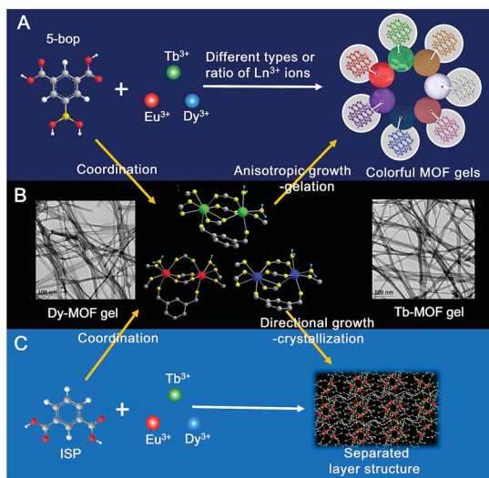
Fig. 1 (A) The selection of different types and ratios of \text{Ln}^{3+} ions for the formation of MOF gels with different colors. (B) The formation of Tb- and Dy-MOF gels because of their different coordination environments compared to that of \text{Eu}^{3+} . (C) Separated layer structure revealed from single crystal results for the formation of nanoribbons, which entangle together to form MOF gels.
