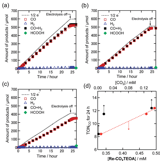
Fig. 4 Time courses of the generation of CO (red square), \text{H}_2 (blue triangle), and formic acid (green diamond) with half of the electrons (dotted line) during bulk electrolysis using the Re(I) catalyst (0.5 mM) at -1.82 \text{ V} in a DMF-TEOA solution containing \text{Et}_4\text{NBF}_4 (0.1 M) under (a) 100%, (b) 10%, and (c) 1% \text{CO}_2 atmospheres ( 10 \text{ mL min}^{-1} ). Total amounts of CO and \text{H}_2 are also indicated by black squares. (d) The relationships of \text{TON}_{\text{CO}} for a 24 h reaction with the concentrations of Re-CO 2 TEOA in the solution (red circle) and \text{CO}_2 (black circle). Corresponding time courses of the current during bulk electrolysis are shown in Fig. S4 † .
