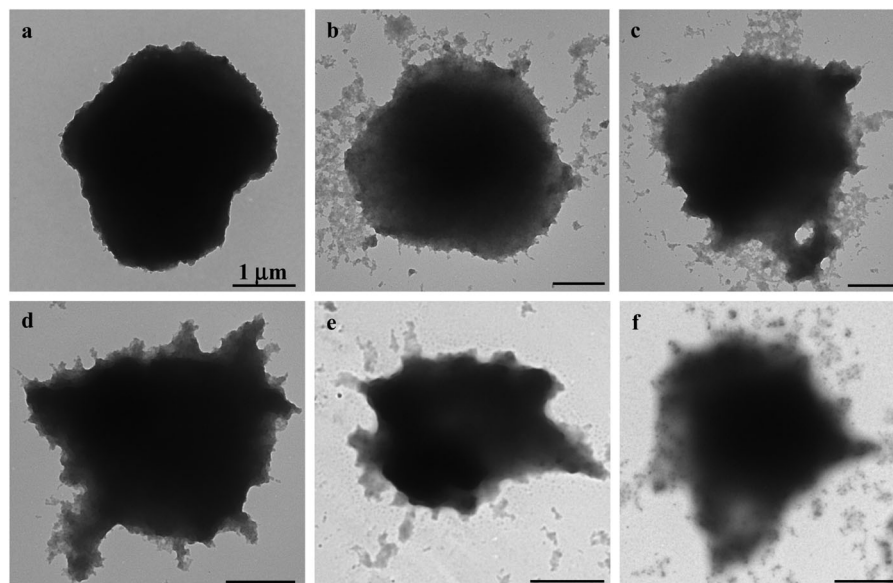
Fig. 2 TEM images showing the process of the protrusion of nanospikes on the surface of CSEG-g-Chol MGs after being incubated in a glutathione solution (5 mM) for 0 (a), 0.5 (b), 1 (c), 3 (d), 12 (e) and 24 h (f), respectively.
