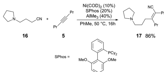
Scheme 5 Activation of alkynitriles using a directing group. 24
