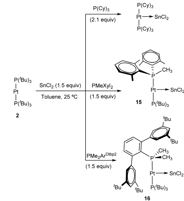
Scheme 5 Tin-mediated phosphine exchange reactions at \text{Pt}(0) 2 .
