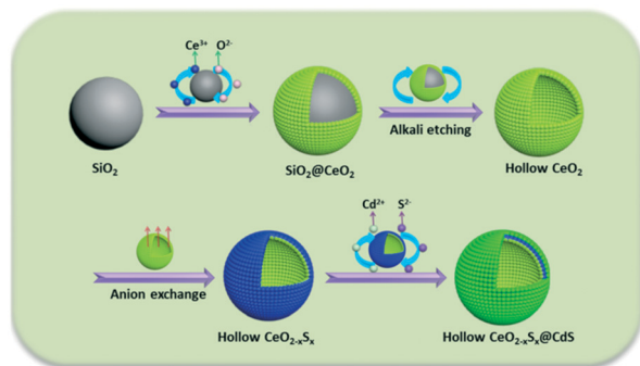
Scheme 1 Schematic illustration for the synthesis of the \text{CeO}_{2-x}\text{S}_x@ CdS composite.
