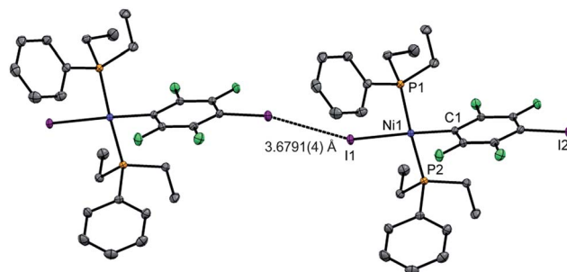
Fig. 2 Molecular structure of 2pl showing intermolecular C-I\cdots I-Ni halogen bond. Displacement ellipsoids at 50% probability level. Hydrogen atoms not shown. A three-molecule chain is illustrated in the ESI.†
