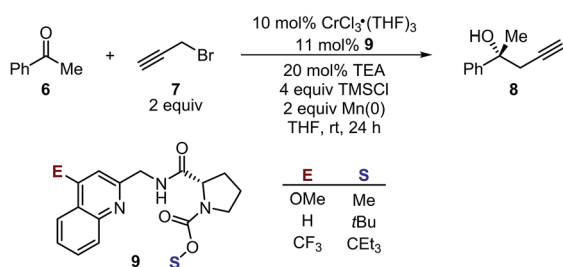
Fig. 2 (A) Desymmetrization of bisphenol. (B) Charton-LFER model. (C) Sterimol-LFER model. (D) Nozaki-Hiyama-Kishi propargylation of acetophenone.
