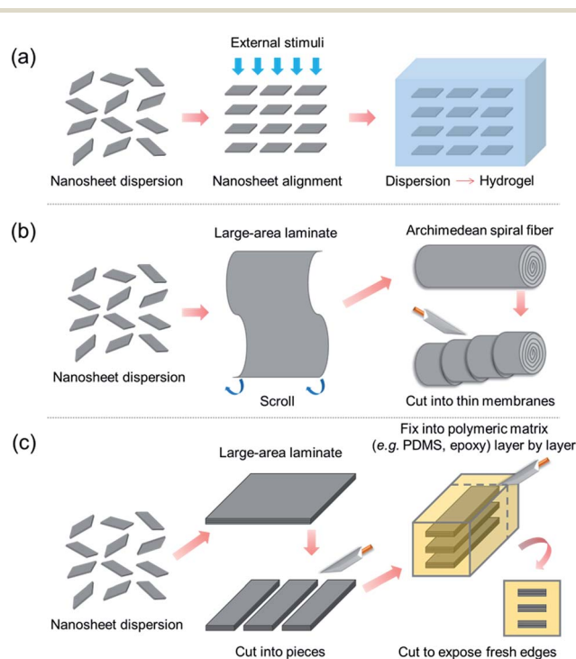
Fig. 7 Schematic diagrams for the proposed strategies to maximize the ultrahigh in-plane ionic conduction of 2D nanosheets. (a) To perpendicularly align and immobilize nanosheets in a matrix by external stimuli. (b) To assemble nanosheets into large-area laminates, scroll into Archimedean spiral fibers and cut into thin pieces perpendicular to the fiber axis. (c) To assemble nanosheets into large-area laminates, cut into pieces and fix them into a polymeric matrix layer by layer, and finally cut again to expose the fresh laminate edges.
