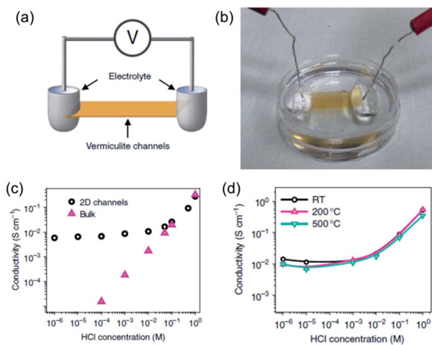
Fig. 4 (a) Schematic drawing and (b) photograph of the experimental setup for measuring the proton conductivity through vermiculite channels. (c) Acid concentration-dependent proton conductivities of vermiculite channels and bulk solutions. (d) Acid concentration-dependent proton conductivities of pristine and 200 °C and 500 °C annealed vermiculite membranes. Reproduced with permission. 30 Copyright 2015, Nature Publishing Group.
